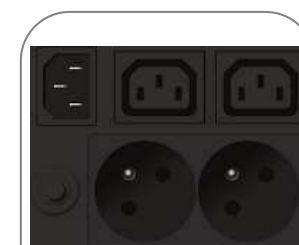
AC Input, fuse, 2x IEC and 2x French outlet
